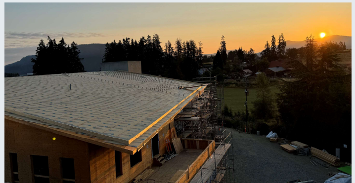
Roof VB complete / steel beam in / insulation clips started
